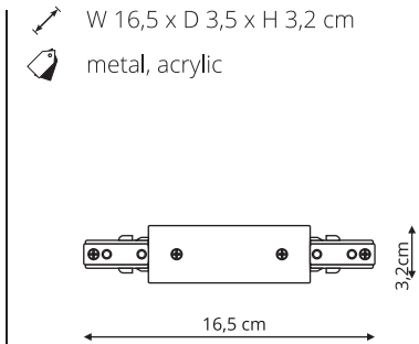
central/internal power supply 3F LP-555-3F white LP-555-3F black
