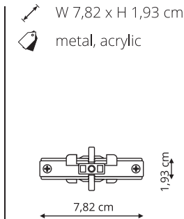
3F internal connector LP-551-3F white LP-551-3F black
